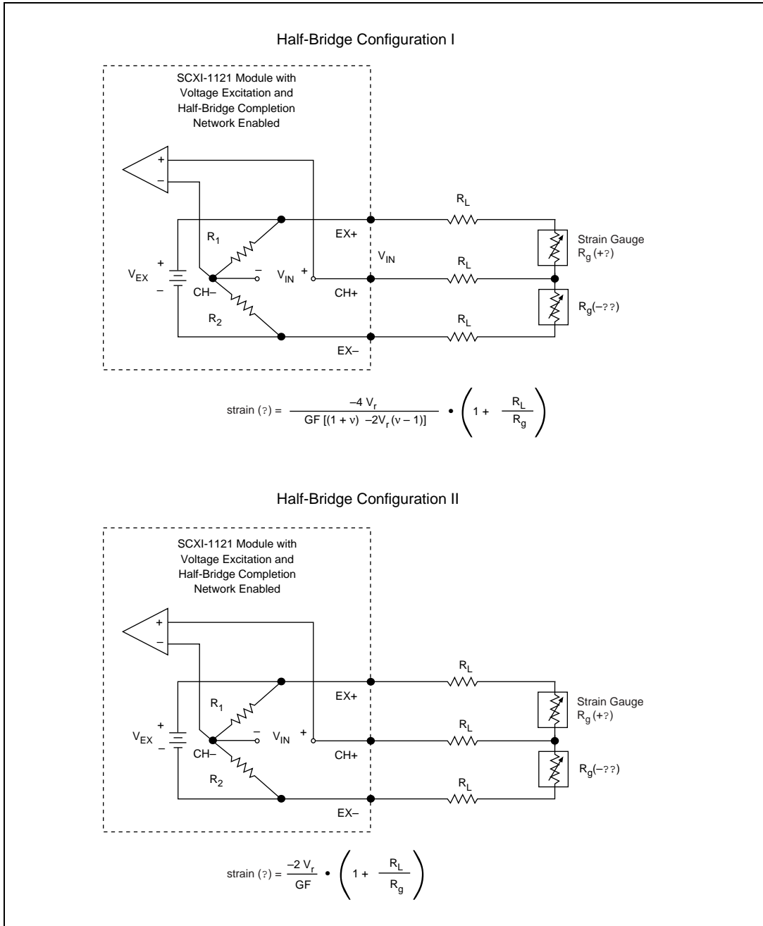
Figure 4-6. Half-Bridge Configurations
