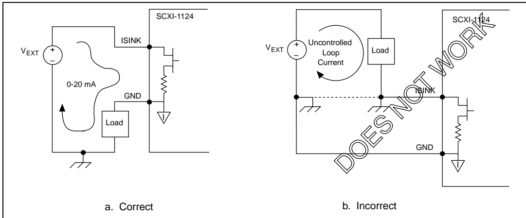
Figure 4-16. Current Loop Connection, Load and External Supply Both Grounded
