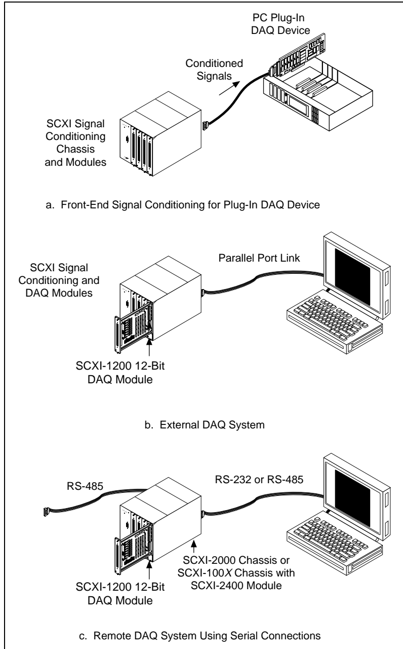
Figure 1-1. SCXI Systems
